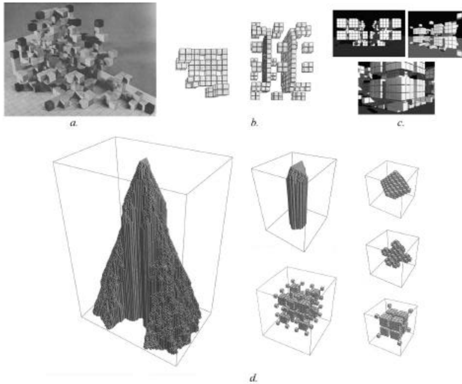
Figure 1. Three-dimensional cellular automata
